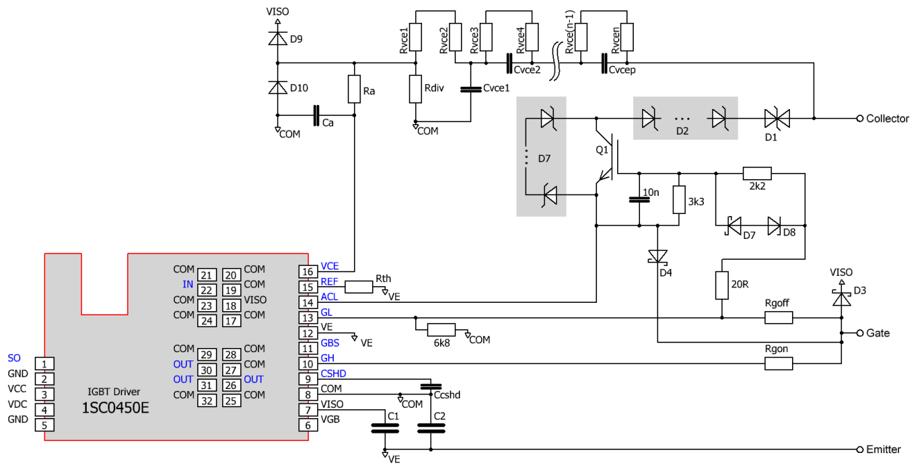
Fig. 6 Recommended user interface of the 1SC0450E2B0 (secondary-side pins 6 to 16) without gate boosting (refer to chapter "Gate Boosting" and Fig. 11 for gate-boosting circuitry)
