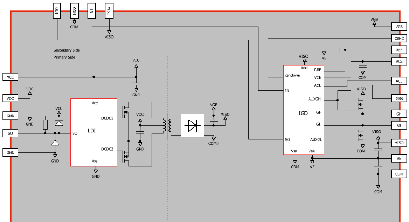
Fig. 2 Block diagram of the 1SC0450E2B0 driver core
