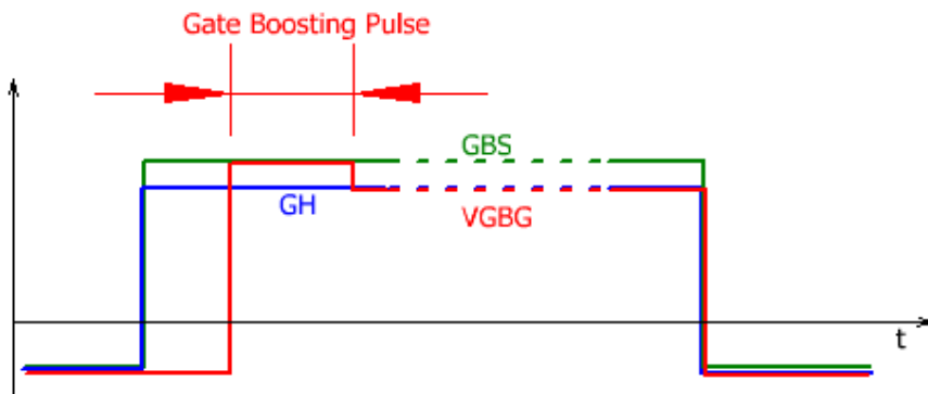
Fig. 11 Gate-boasting circuit principle – highlighted in red color
